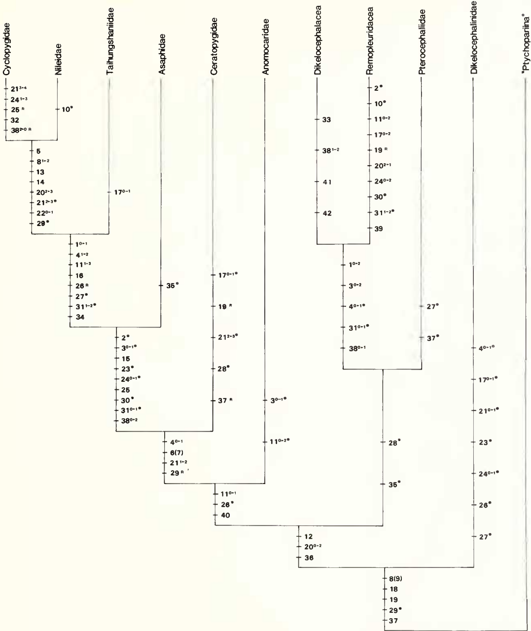
TEXT-FIG. 3. Another cladogram produced from the PAUP computer analysis of the characters given in Table 2, equally parsimonious with that shown on text-fig. 2. *, characters which are developed in parallel in more than one place on the cladogram; R, character reversals (i.e. advanced to primitive on Table 2); +, character transformations which we consider unlikely on other evidence (see text).
